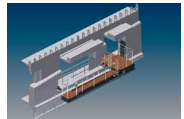
Accommodation ladder
