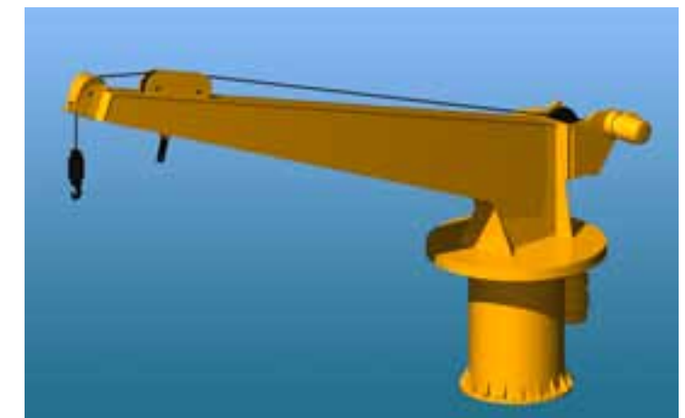
FWSC 50 kN with hydraulic wave compensation
